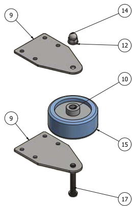
RIGHT EXTENDER
