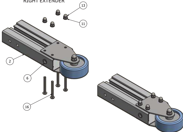
RIGHT EXTENDER
