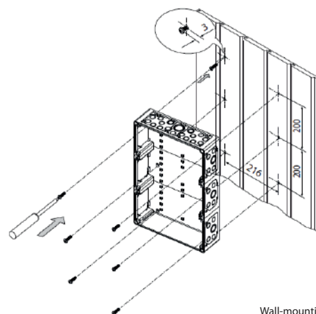
Wall-mounting installation
