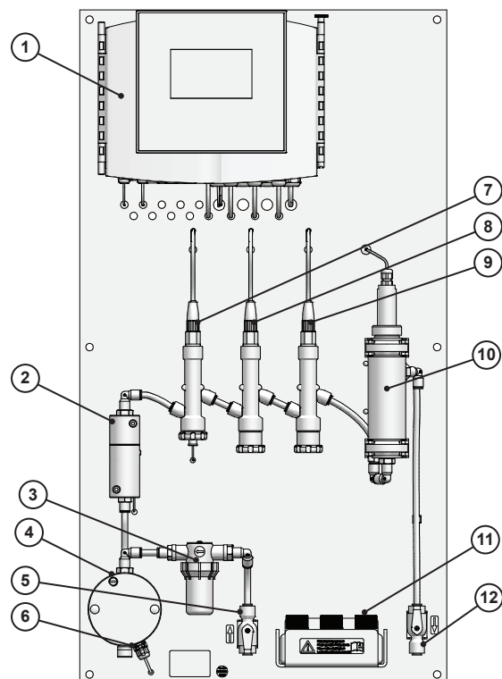
Figur 2: Vandanalysepanel EASYPRO 4
