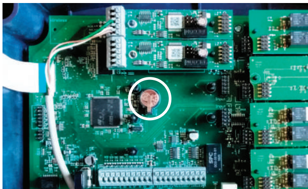
Figur 36: Knapcellebatteri R1220
