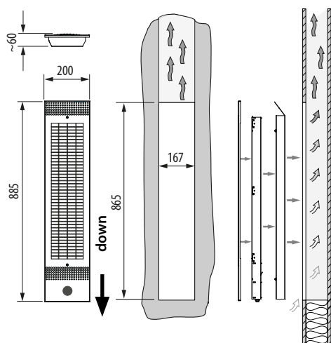
Front view Wall cut-out with rear ventilation
